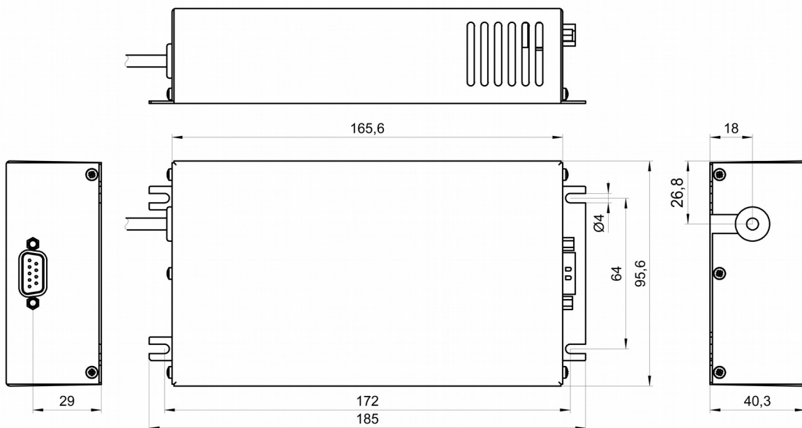
Figure 4: dimensional drawing CPS 30kV
