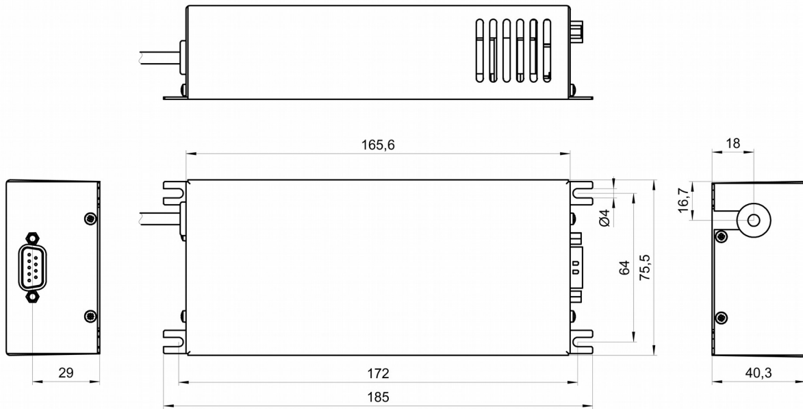
Figure 3: dimensional drawing CPS 10kV - 20kV
