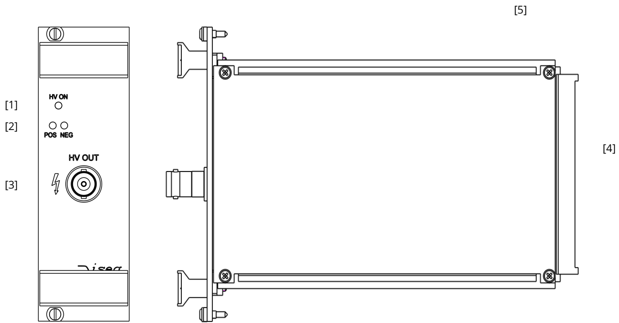
Figure 4: Front view
