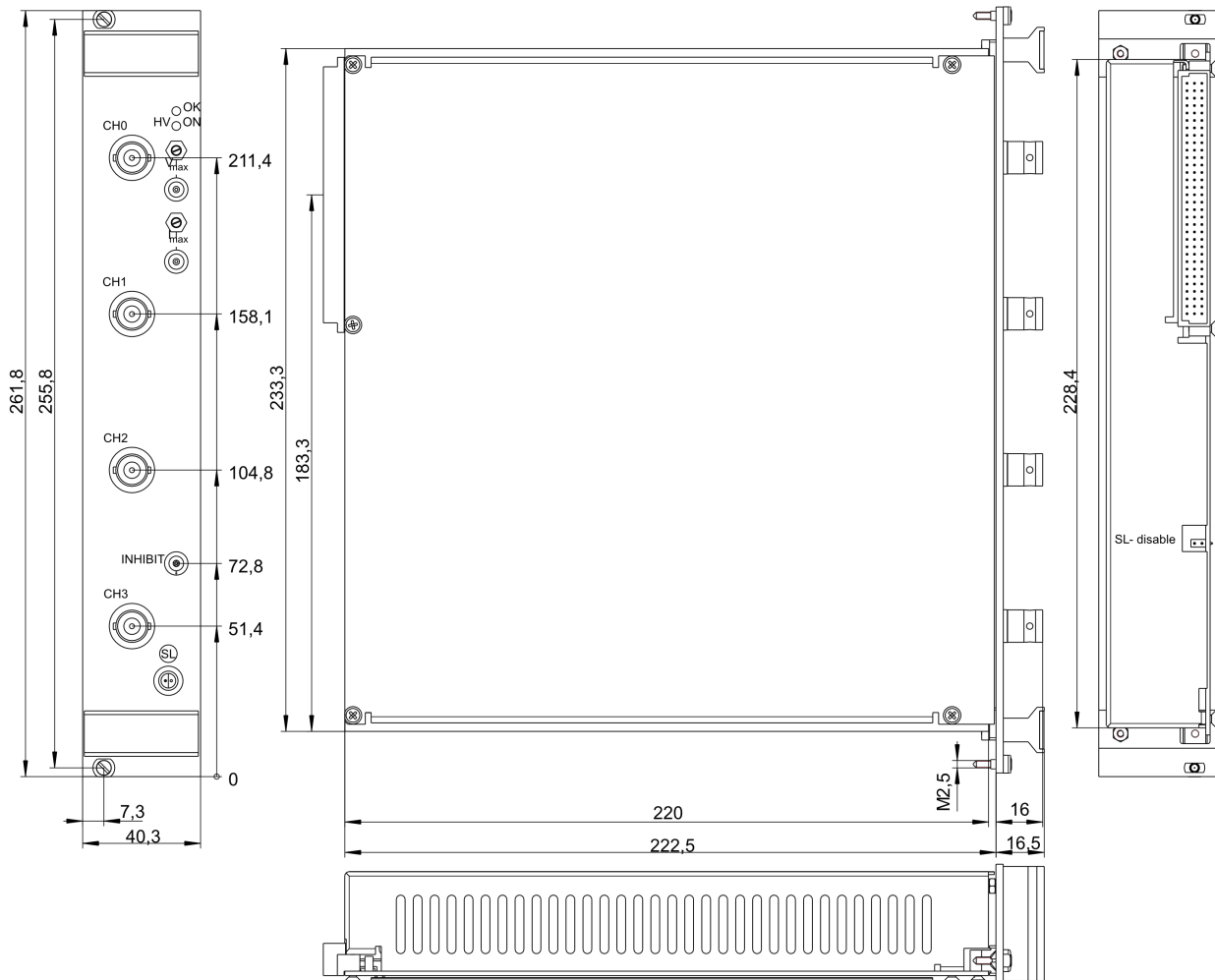
Figure 2: 4 channels with SHV in Floating Ground / Common Floating Ground
