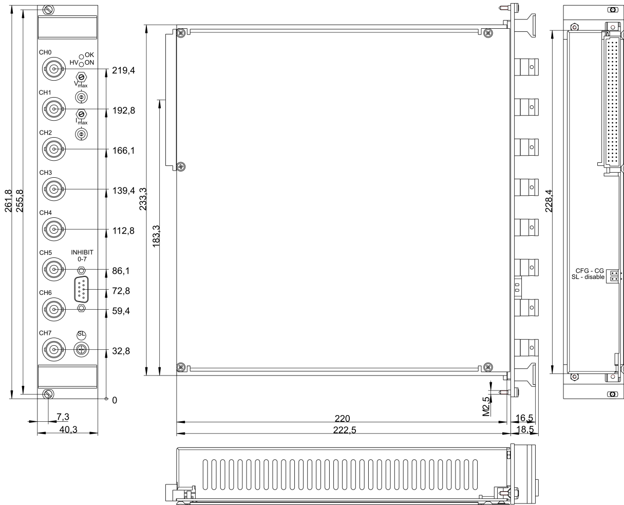
Figure 6: 8 channels with SHV in Floating Ground or Common Floating Ground and Inhibit
