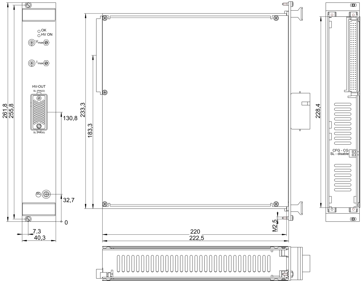
Figure 10: 8, 16, 48 channels in Floating Ground or Common Floating Ground with Redel
