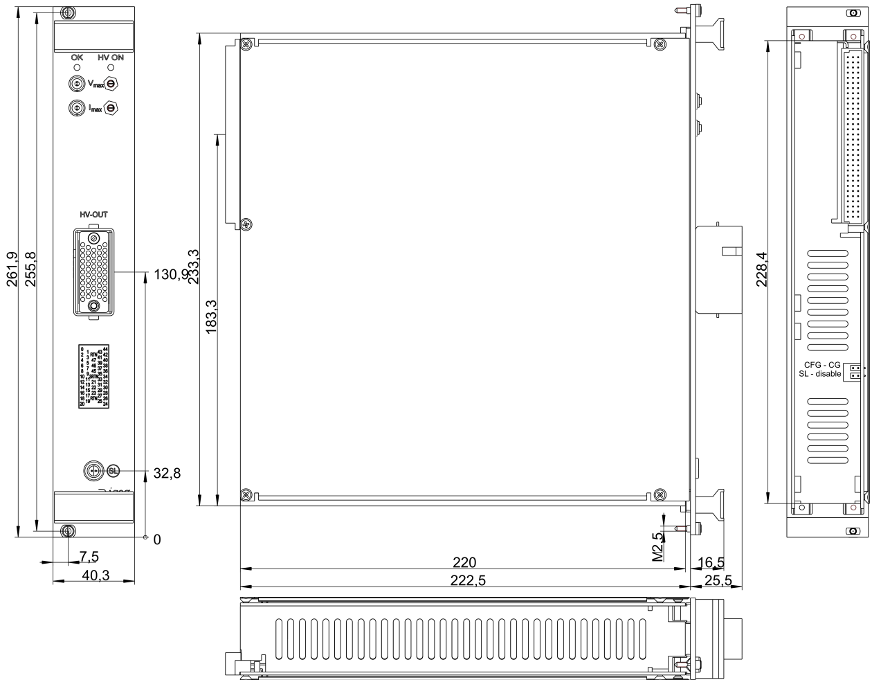
Figure 12: 16, 24, 48 channels in FLEX with Redel
