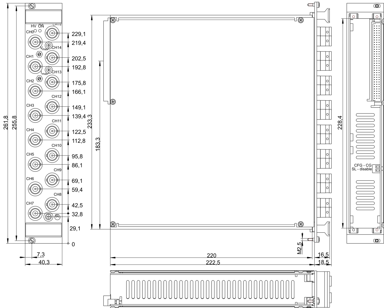
Figure 7: 16 channels with SHV in Common Ground
